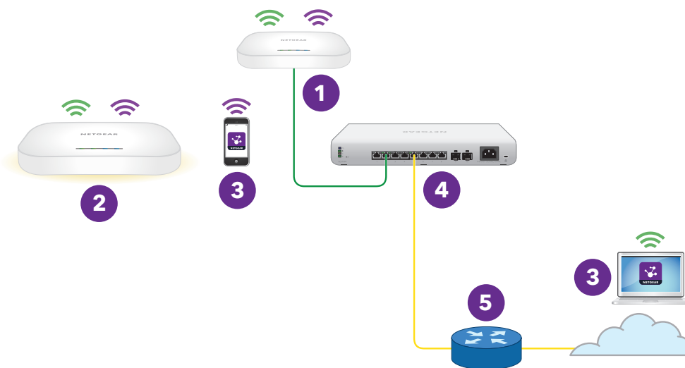
Figure 9. Mesh network with an extender access point and a wired root access point
