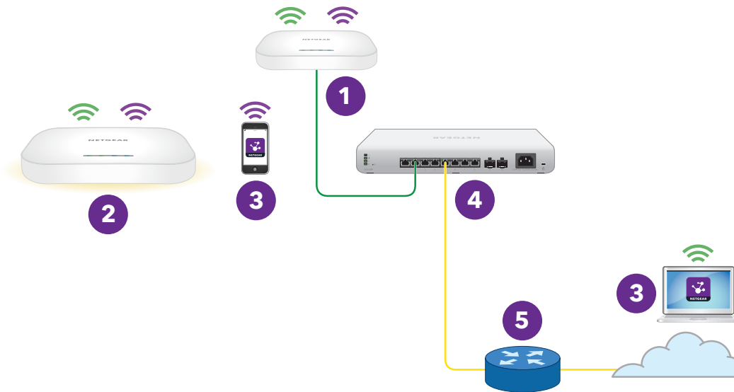
Figure 11. Connect the extender access point to a wired root access point
