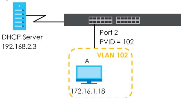
Figure 52 Tutorial: DHCP Relay Scenario
