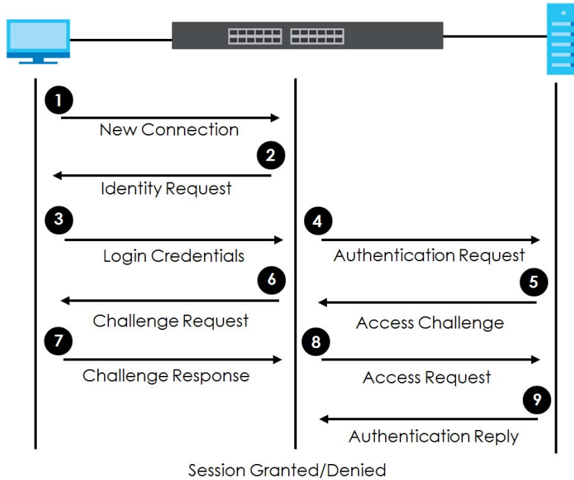
Figure 134 IEEE 802.1x Authentication Process
