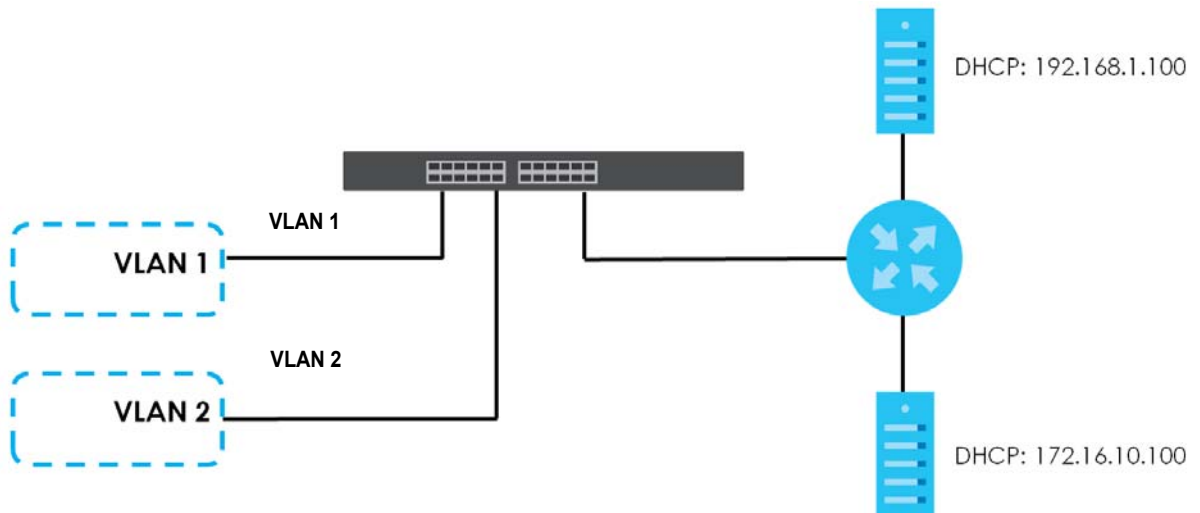
Figure 248 DHCP Relay for Two VLANs
