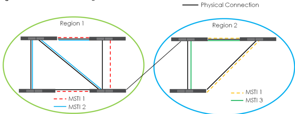
Figure 124 MSTIs in Different Regions
