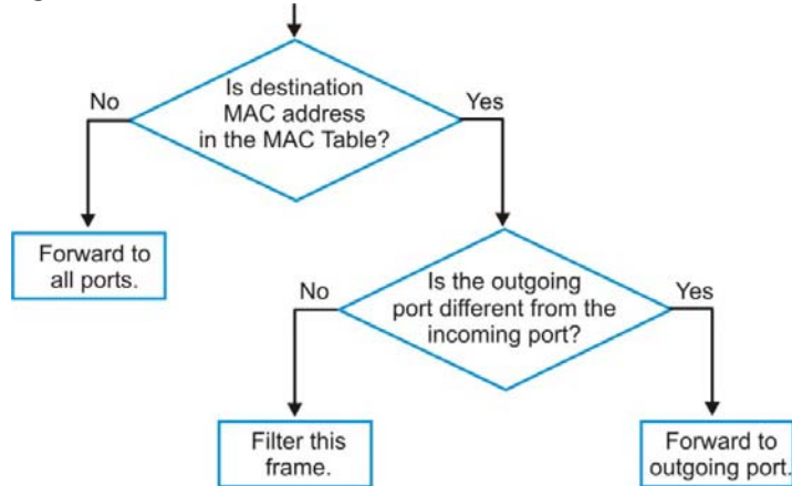
Figure 292 MAC Table Flowchart
