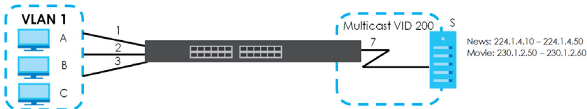
Figure 166 MVR Configuration Example
