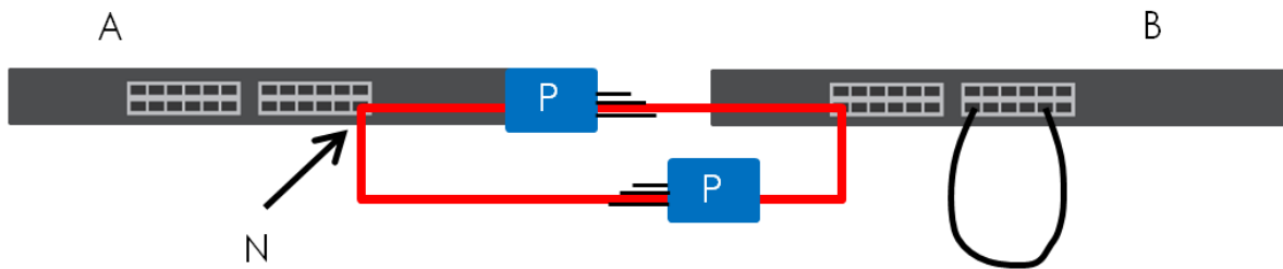
Figure 193 Loop Guard – Probe Packet
