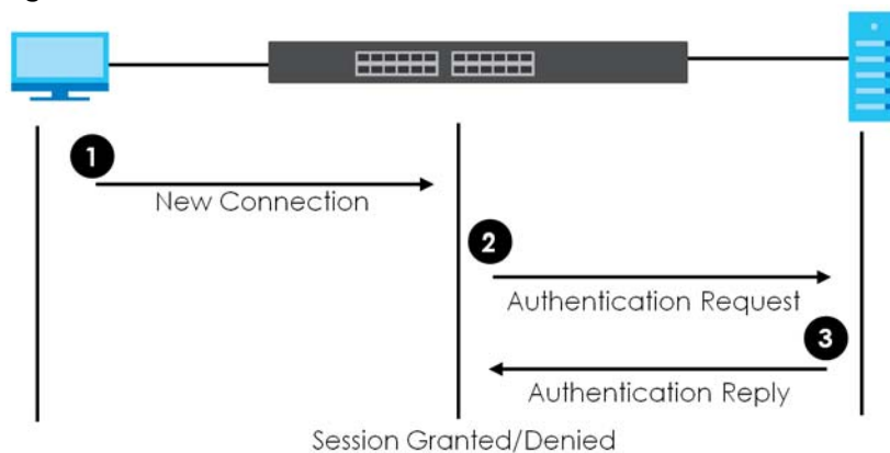
Figure 135 MAC Authentication Process
