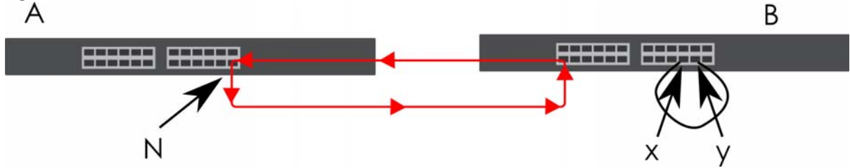
Figure 192 Switch in Loop State
