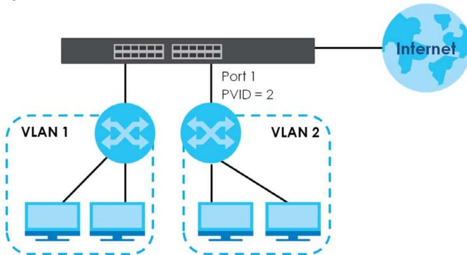
Figure 43 Initial Setup Network Example: Port VID
