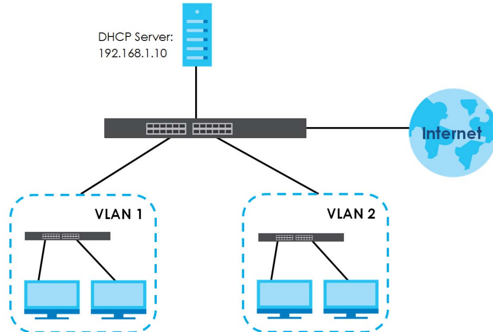
Figure 244 Global DHCP Relay Network Example
