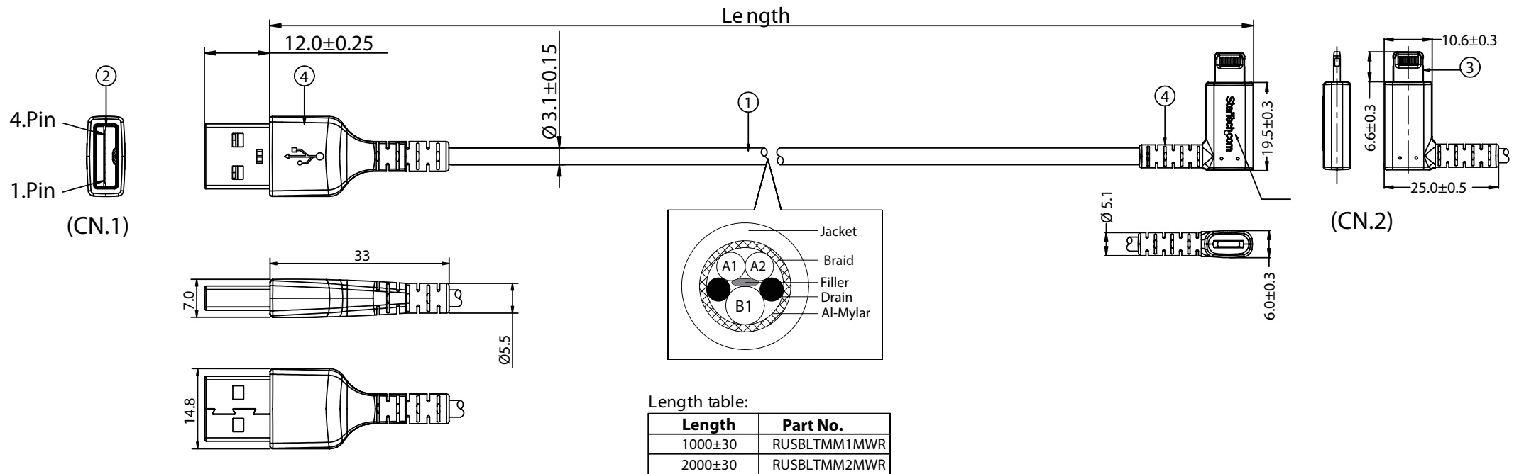
(A). Wire Pin Assignment and Wire Description.
