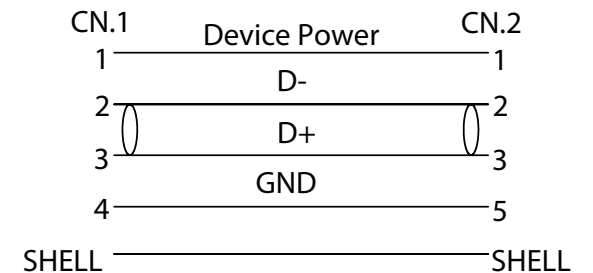
(A). Wire Pin Assignment and Wire Description.
